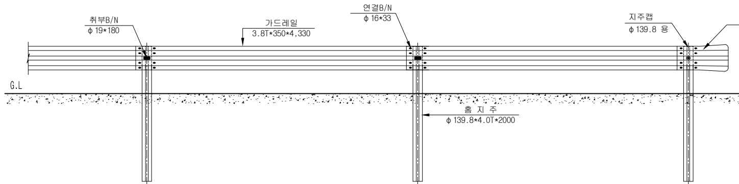
RAIL ELEVATION SCALE: NONE
