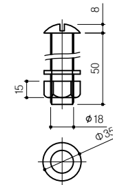
SETTING B/N (φ18*50)
