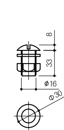
JOINTING B/N (φ16*33)
