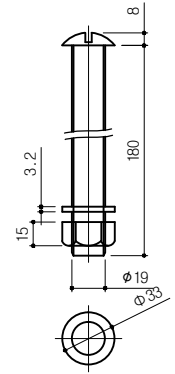
SETTING B/N (φ19*180)
